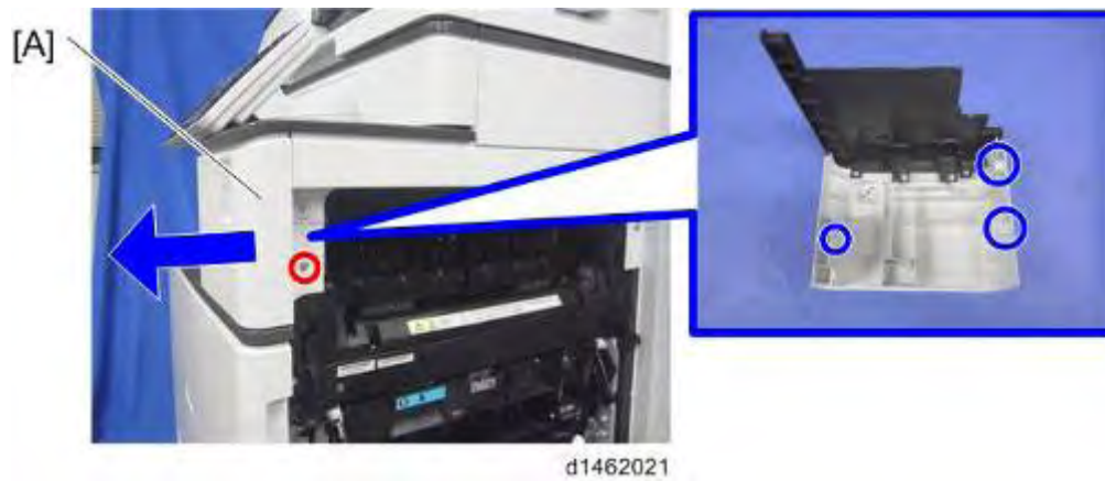
10. Paper output cover [A] (⌀×1).
