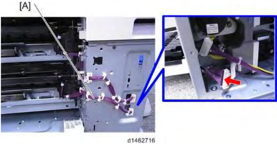
13. 2nd Paper feed unit [A] (2x)
