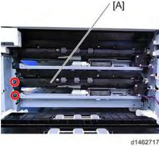
13. 2nd Paper feed unit [A] (2x)
